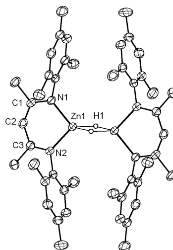
Fig. 1. Molecular structure of the P \bar{1} polymorph of 1 in the crystal ( 1a ). The molecule has a crystallographically imposed center of inversion.
