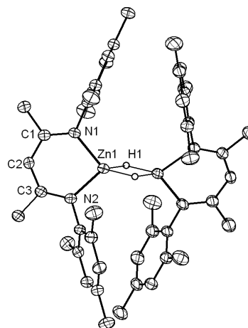
Fig. 2. Molecular structure of the P2 / n polymorph of 1 in the crystal ( 1b ). The molecule has a crystallographically imposed C 2 axis.
